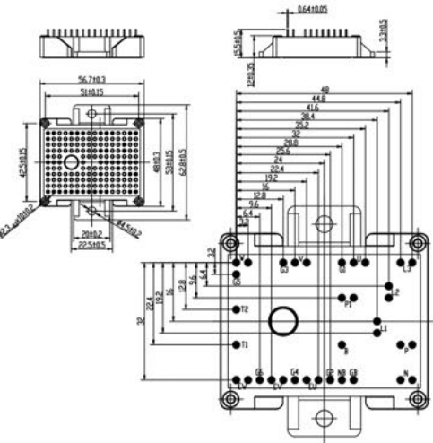
Pinpositions with tolerance \pm 0.1 L3.1
