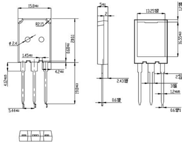
TO-247PLUS-3L
