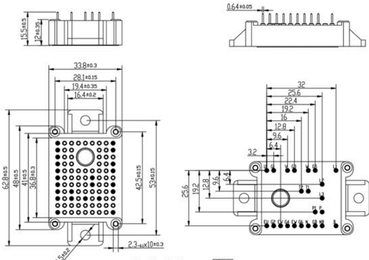
Pinpositions with tolerance \pm 0.1 L2.1
