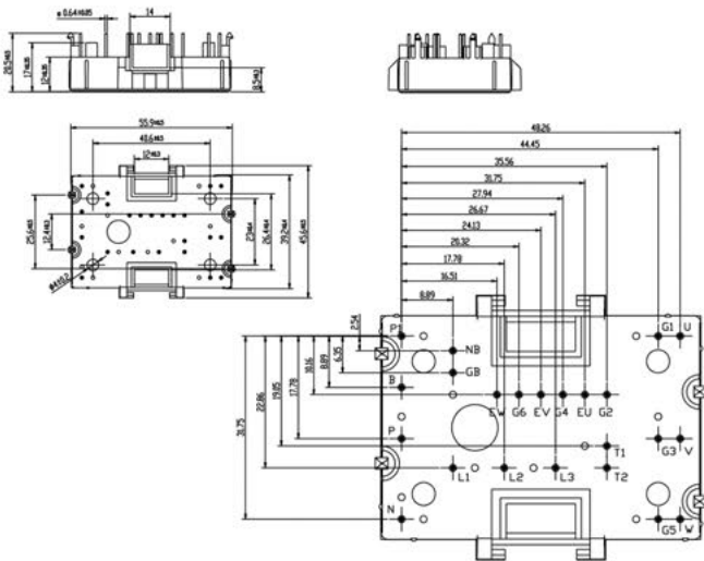
Pinpositions with tolerance \pm 0.1 L1.0
