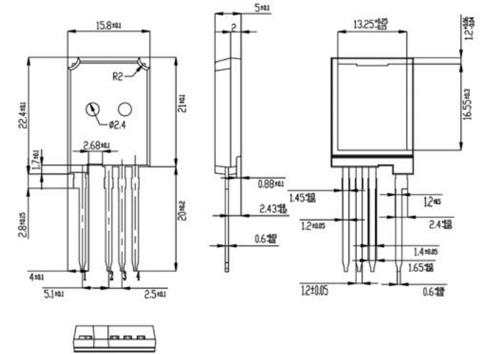
TO-247PLUS-4L
